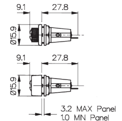
Fixing Details
