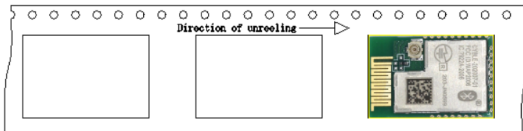
Figure 12. Component Orientation in Tape and Unreeling Direction (Illustration Only)
