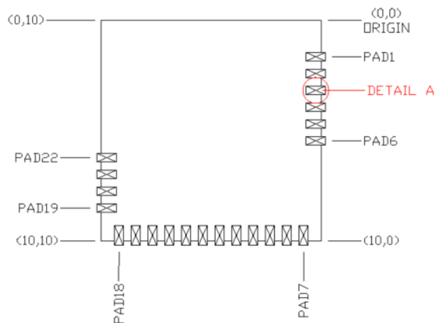
Top View (Seen on Host PCB)
