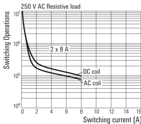
Electrical service life 230 V AC resistive load 230 V AC resistive load
