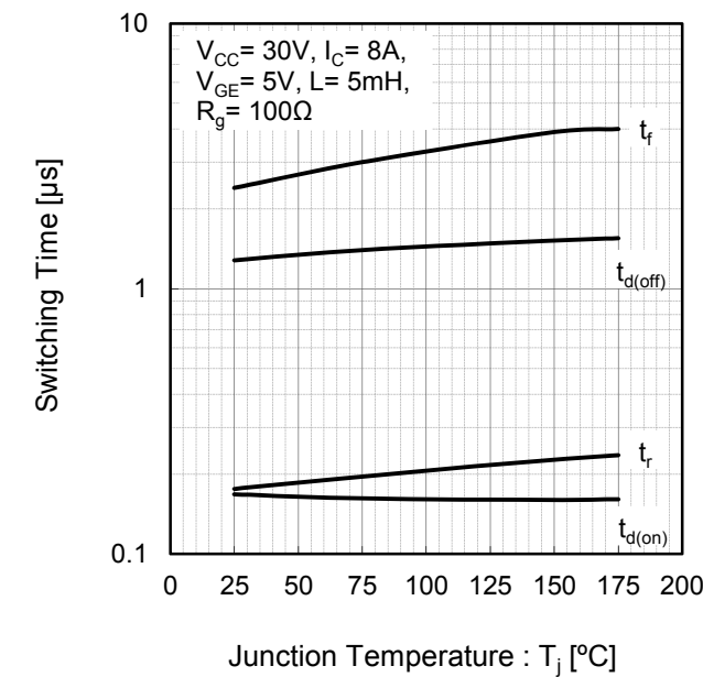
Fig.13 Typical Switching Time vs. Junction Temperature
