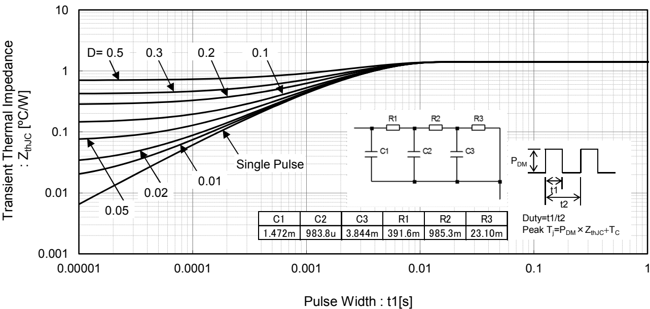
Fig.14 Transient Thermal Impedance
