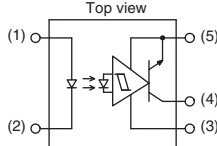
Internal circuit
