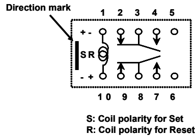
Single coil latch type
