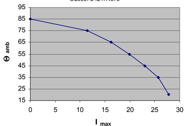
Max. allowable ambient Temp. at specific current (rms) B25667C4247A375
