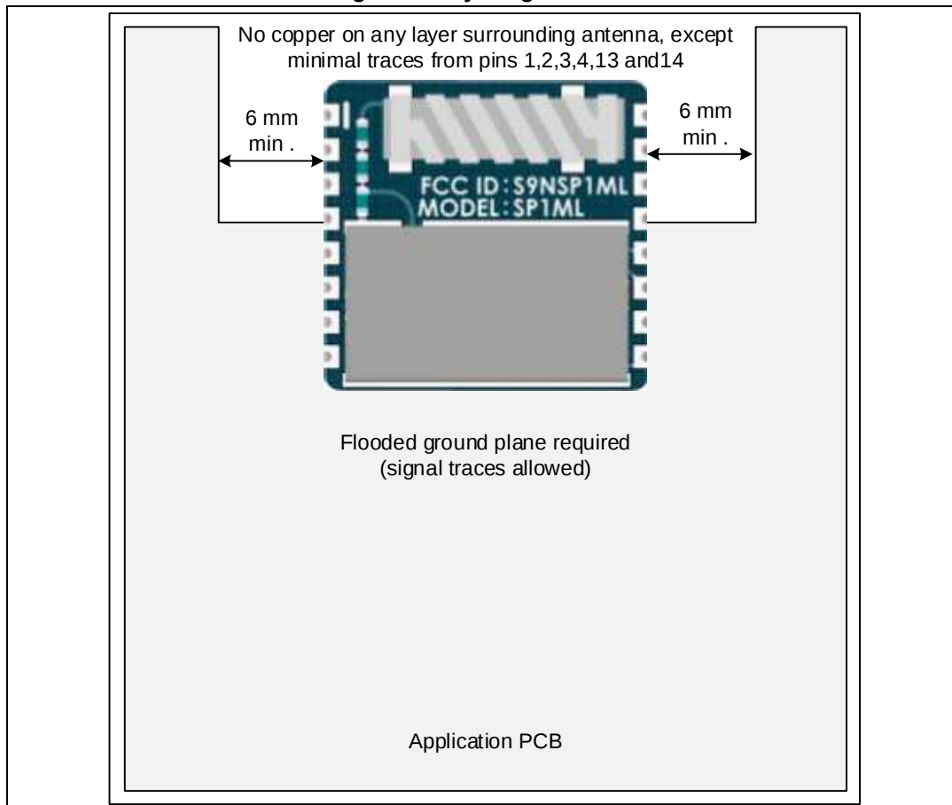
Figure 5. Layout guidelines
