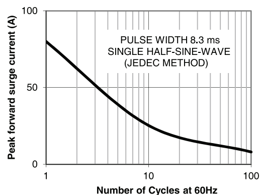
Figure 2. Maximum NON-Repetitive
