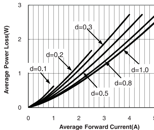
Figure 6. Forward Power Loss Characteristics
