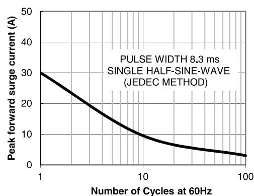
Figure 2. Maximum NON-Repetitive
