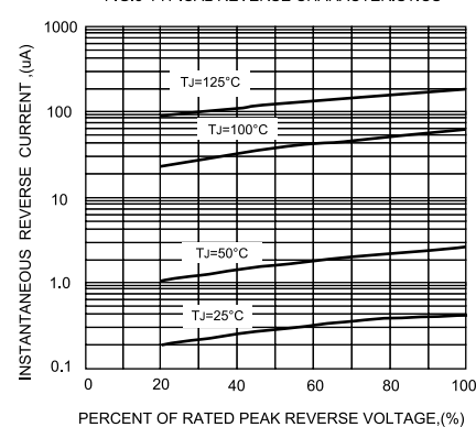
FIG.5-TYPICAL REVERSE CHARACTERISTICS
