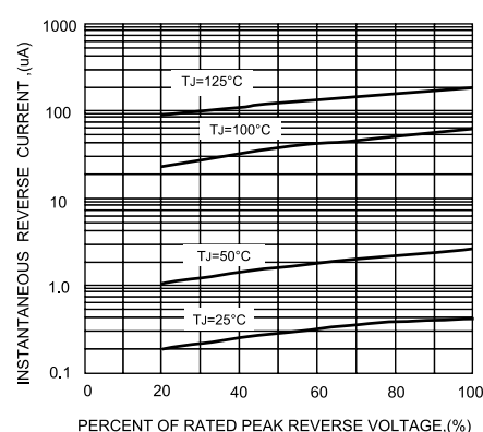
FIG.5-TYPICAL REVERSE CHARACTERISTICS
