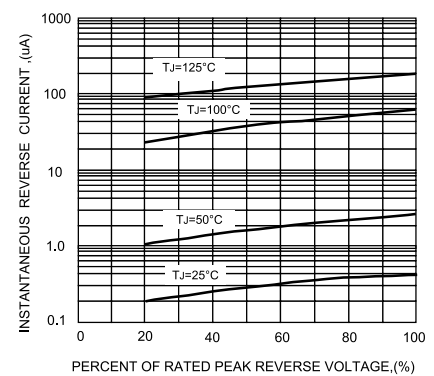
FIG.5-TYPICAL REVERSE CHARACTERISTICS
