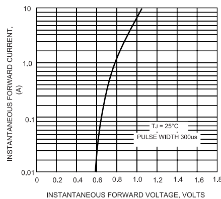
FIG.4-TYPICAL FORWARD CHARACTERISTICS
