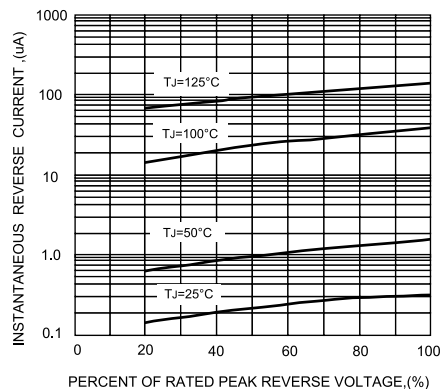
FIG.5-TYPICAL REVERSE CHARACTERISTICS
