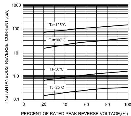
FIG.5-TYPICAL REVERSE CHARACTERISTICS
