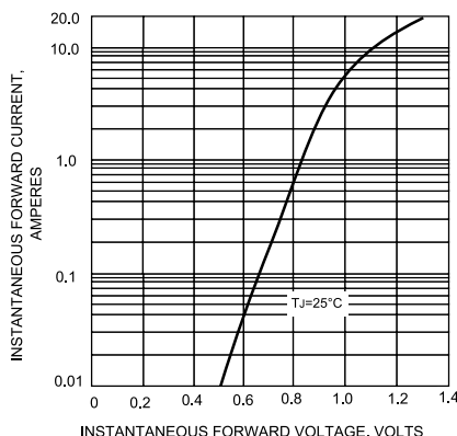
FIG.4-TYPICAL FORWARD CHARACTERISTICS
