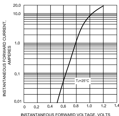
FIG.4-TYPICAL FORWARD CHARACTERISTICS
