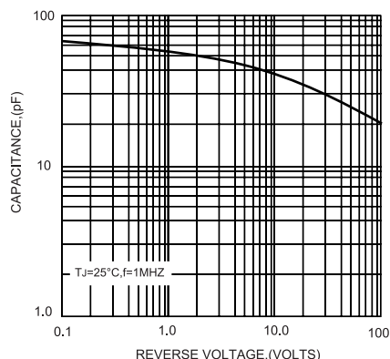
FIG.3-TYPICAL JUNCTION CAPACITANCE
