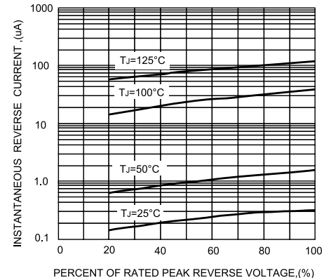
FIG.5-TYPICAL REVERSE CHARACTERISTICS
