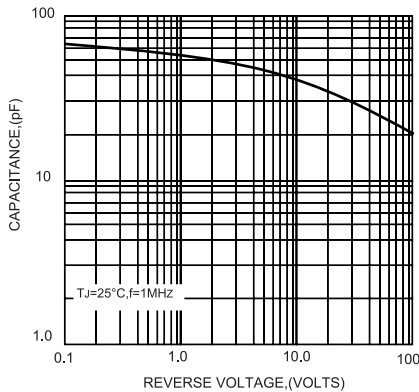
FIG.3-TYPICAL JUNCTION CAPACITANCE
