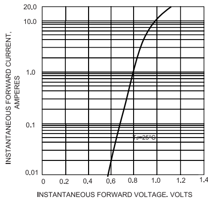
FIG.3-TYPICAL FORWARD CHARACTERISTICS
