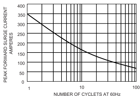
FIG.1-MAXIMUM FORWARD SURGE CURRENT
