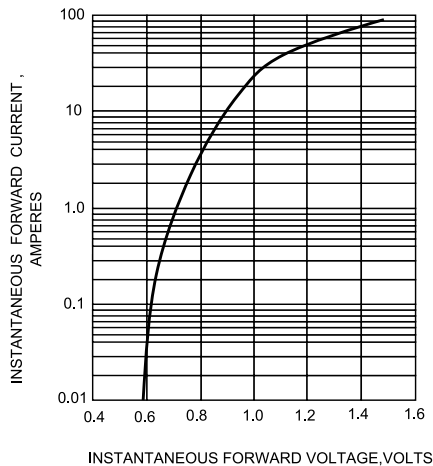
FIG.3-TYPICAL FORWARD CHARACTERISTICS
