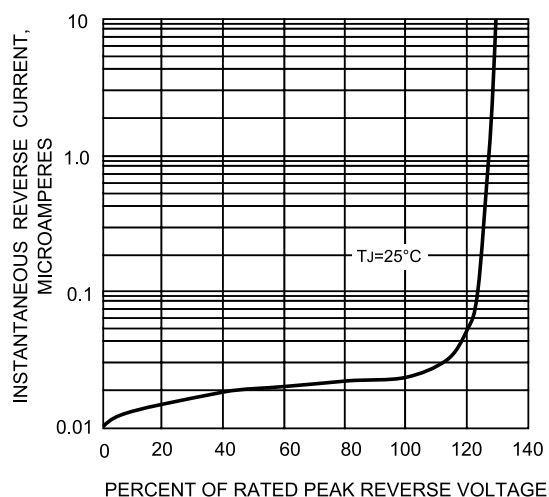
FIG.4-TYPICAL REVERSE CHARACTERISTICS
