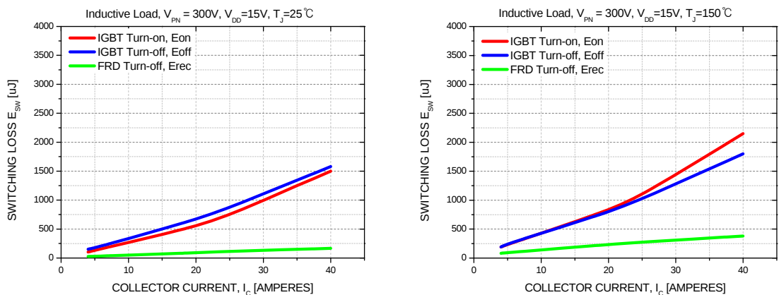
Figure 6. Switching Loss Characteristics
