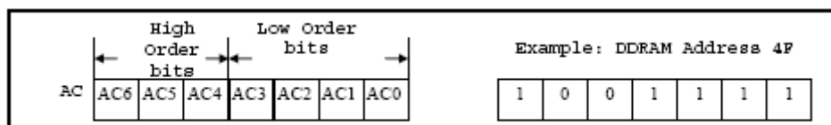
Figure 1 DDRAM Address
