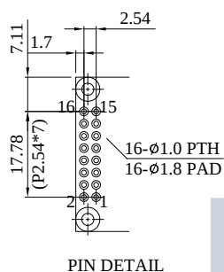
PIN DETAIL
