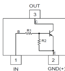
Device Schematic
