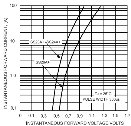
FIG.3-TYPICAL FORWARD CHARACTERISTICS
