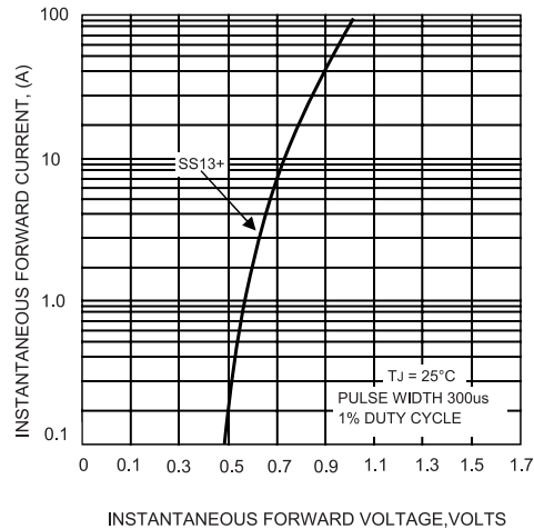
FIG.3-TYPICAL FORWARD CHARACTERISTICS
