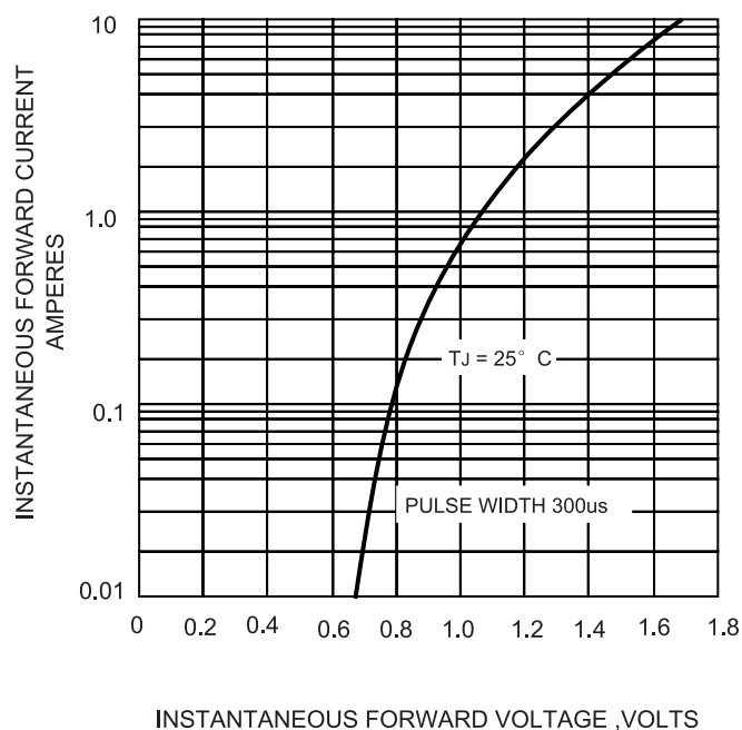
FIG.4-TYPICAL FORWARD CHARACTERISTICS
