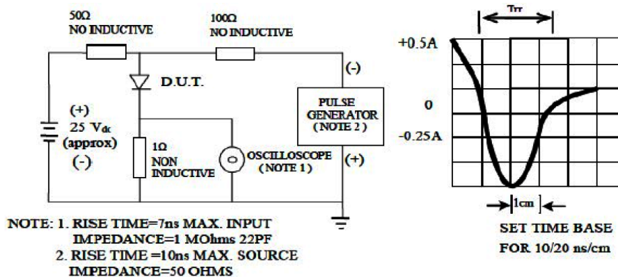
FIG.5 - REVERSE RECOVERY TIME CHARACTERISTIC AND TEST CIRCUIT
