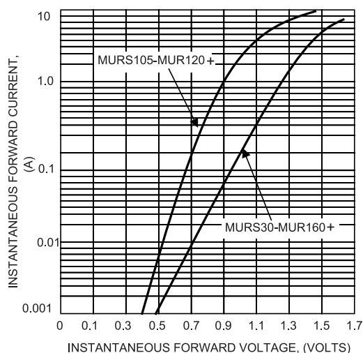
FIG.3-TYPICAL FORWARD CHARACTERISTICS
