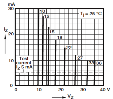
Breakdown Characteristics
