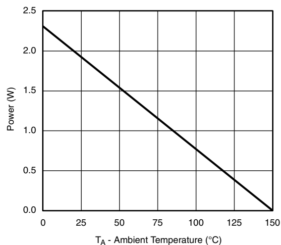
Power, Junction-to-Ambient
