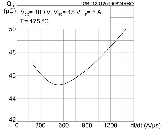
Figure 23: Reverse recovery charge vs. diode current slope
