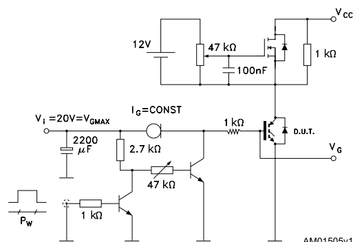
Figure 27: Gate charge test circuit
