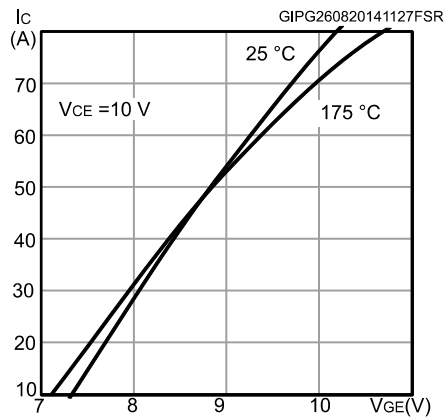
Figure 4: Transfer characteristics
