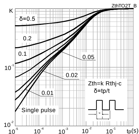
Figure 25: Thermal impedance
