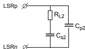
Figure 31: Load circuit B: Piezo loudspeaker
