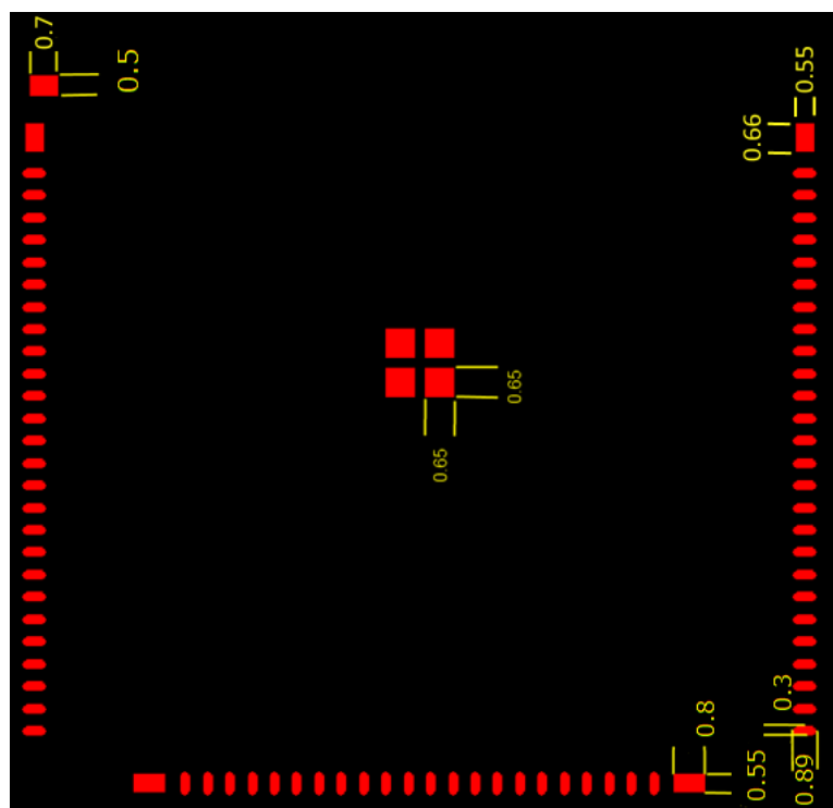
Figure 42: Solder stencil
