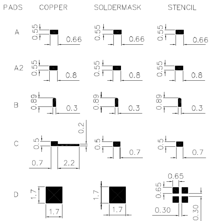
Figure 41: Copper pad, Solder mask opening and Stencil
