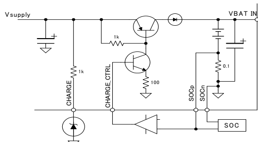
Figure 18: Handset (PP) application with 2x NiMH
