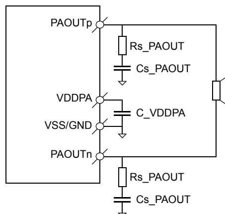
Figure 9: Loudspeaker connection
