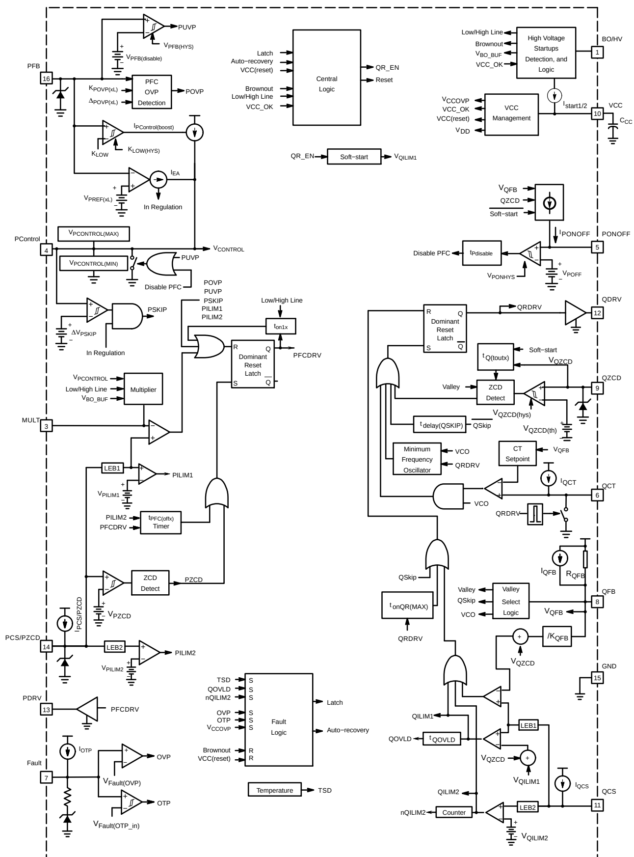
Figure 2. NCL30030 Functional Block Diagram
