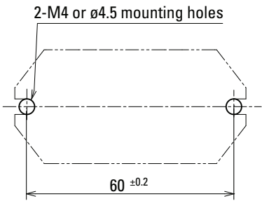
Flange Mount
