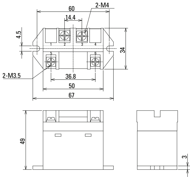
RL1N-T Screw Terminal 1 Pole Flange Mount
