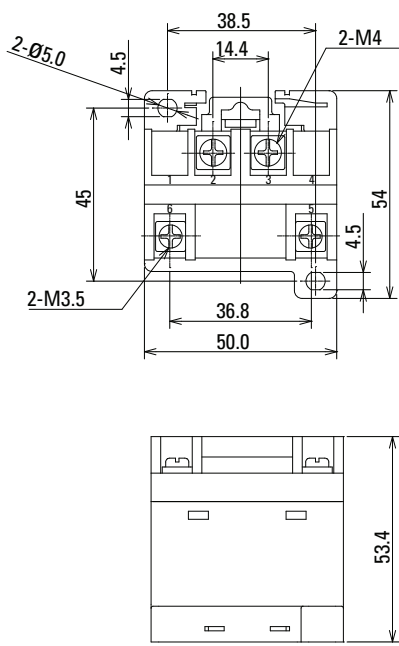
RL1N-D Screw Terminal 1 Pole DIN Rail Mount
