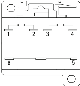
Quick Connect Terminal 2 Pole DIN Rail Mount
