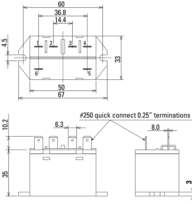
RL2B-T Quick Connect Terminal 2 Pole Flange Mount
