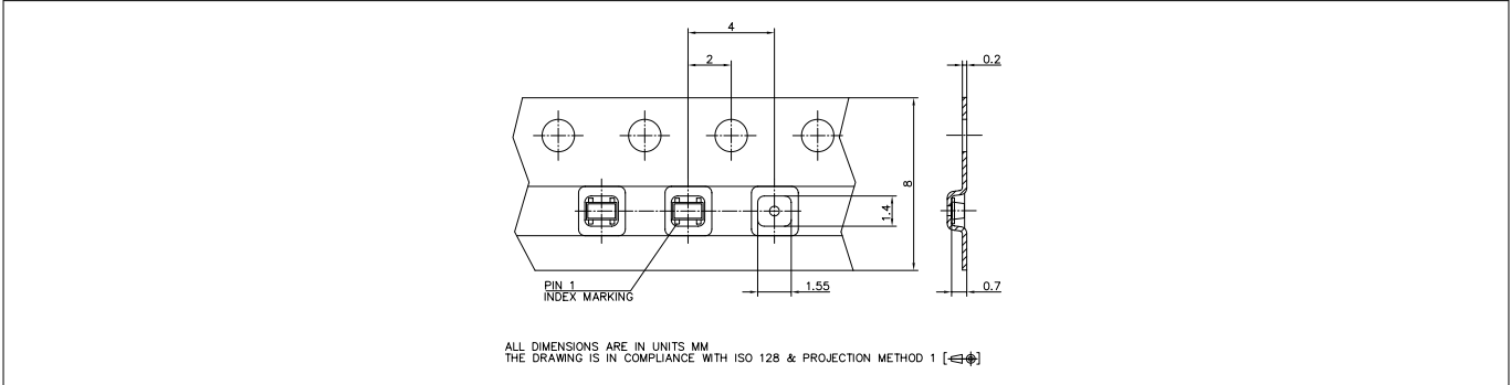
Figure 18 Tape dimensions
