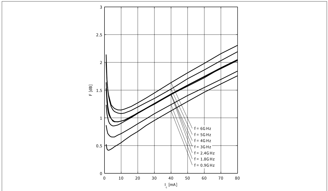
Figure 13 Noise figure NF_{min} = f(I_c) , Z_S = Z_{S,opt} , V_{CE} = 1.5\text{ V} , f = \text{parameter in GHz}
