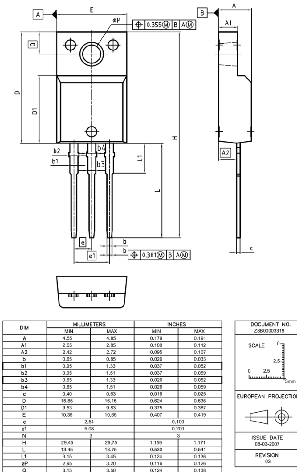
Figure 2 Outlines TO-220 FullPAK, dimensions in mm/inches
