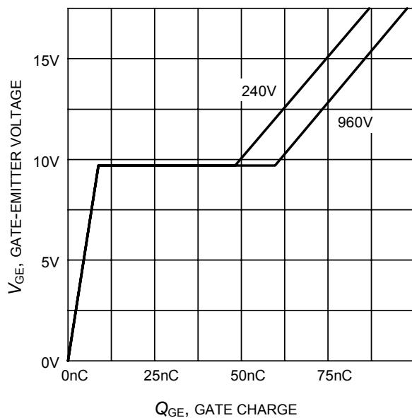
Figure 17. Typical gate charge ( I_C = 25 A)
