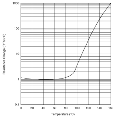
Resistance-Temperature Charac.
