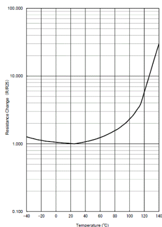
Resistance-Temperature Charac.
