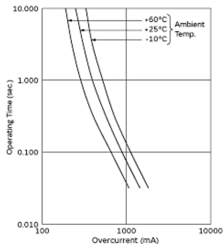
Operating Time (Typical Curve)
