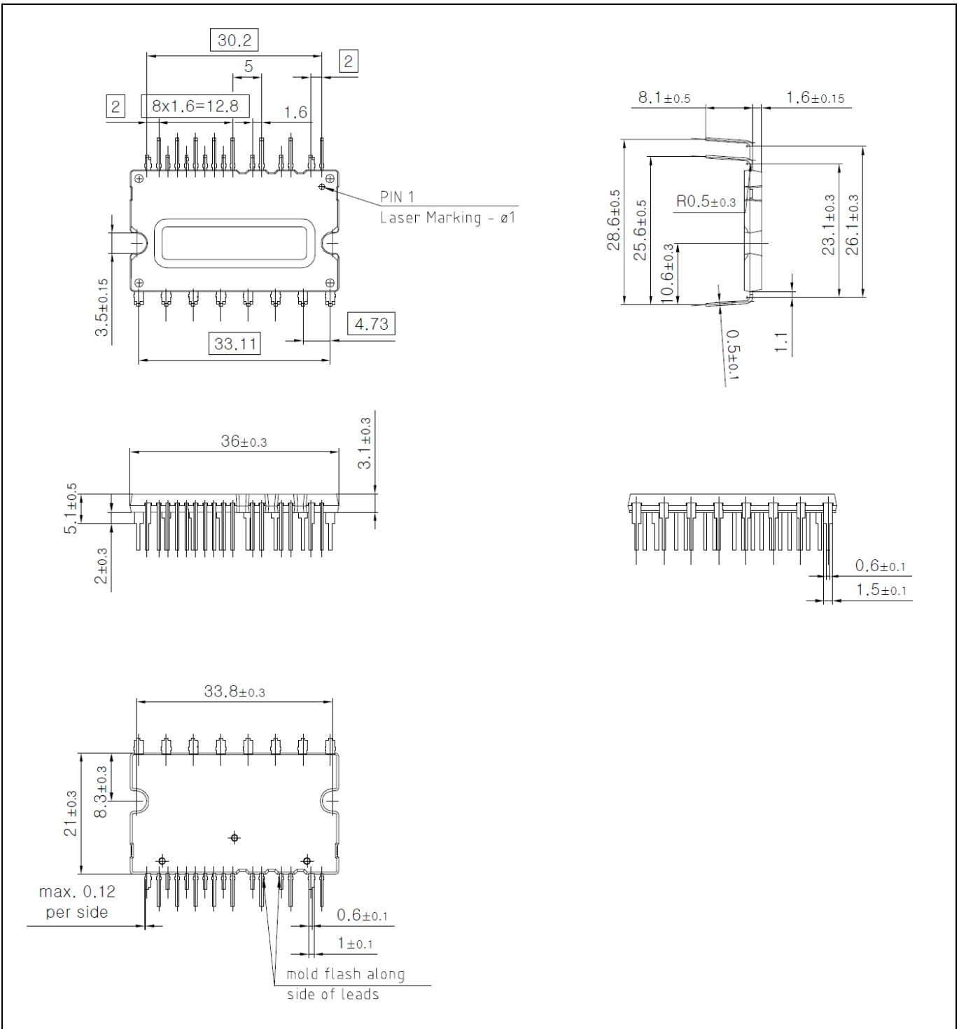
Figure 12 IGCM06F60GA
