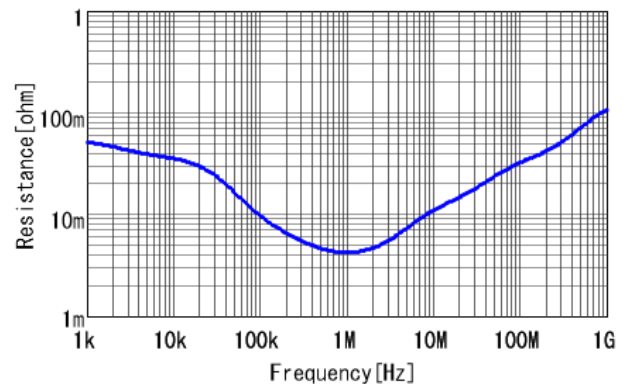
Frequency CharacteristicR
