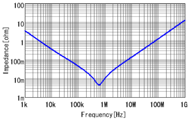
Frequency Characteristic|Z|
