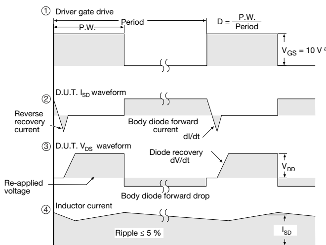
Fig. 20 - For N-Channel
