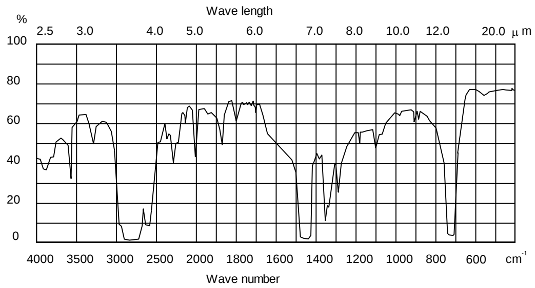
Figure 4. Transmittance
