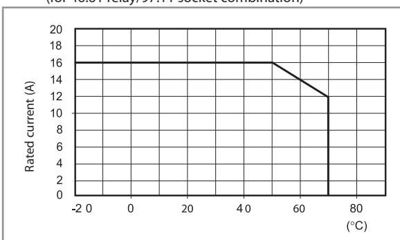
L 97 - Rated current vs ambient temperature (for 46.61 relay/97.11 socket combination)
