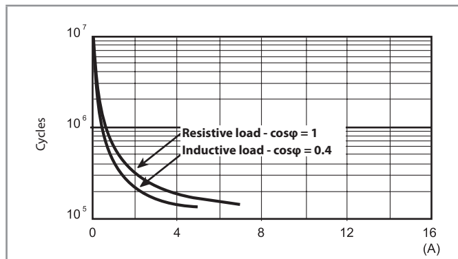
F 58 - Electrical life (AC) v contact current
