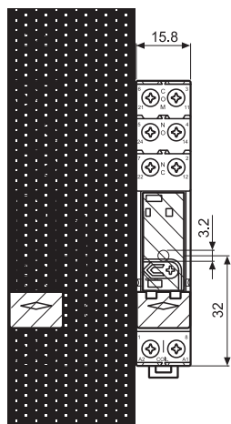
4C.01 / 4C.02 Screw terminals
