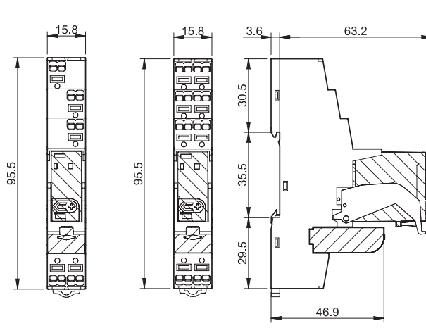
4C.P1 / 4C.P2 Push-in terminals
