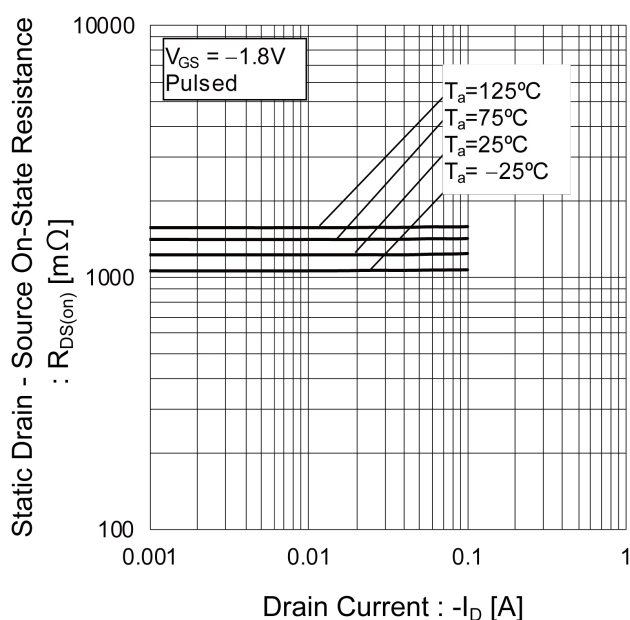
Fig.33 Static Drain - Source On - State Resistance vs. Drain Current (IV)
