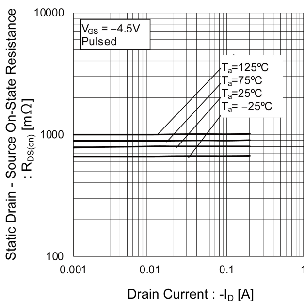
Fig.31 Static Drain - Source On - State Resistance vs. Drain Current (II)
