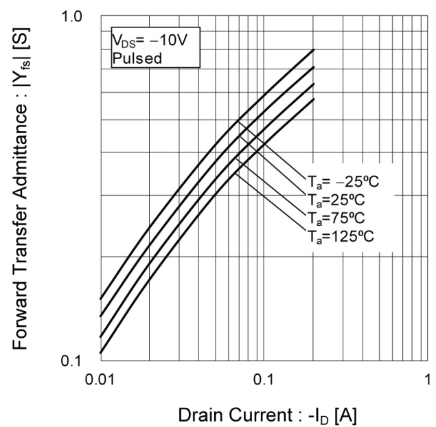
Fig.27 Forward Transfer Admittance vs. Drain Current
