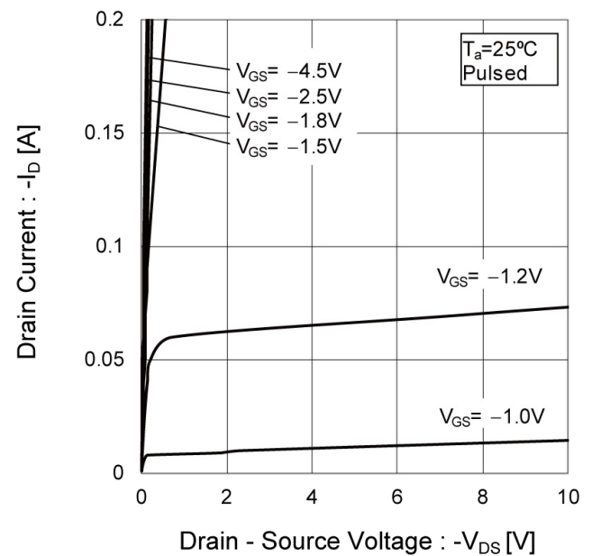
Fig.23 Typical Output Characteristics(II)
