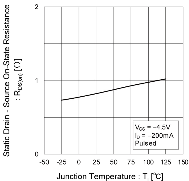
Fig.29 Static Drain - Source On - State Resistance vs. Junction Temperature
