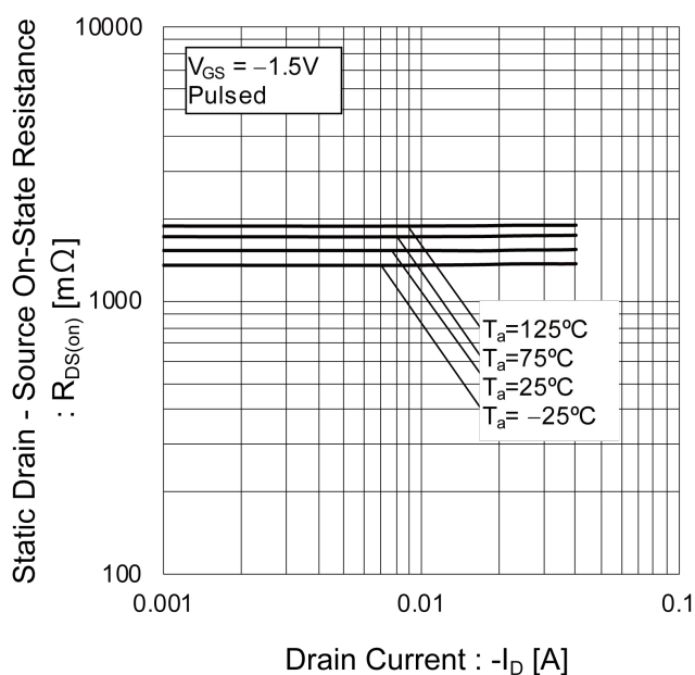
Fig.34 Static Drain - Source On - State Resistance vs. Drain Current (V)
